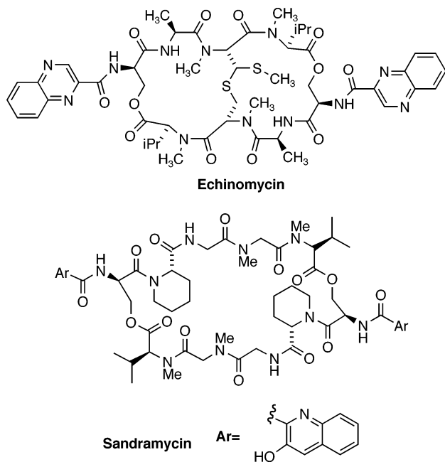
FIGURE 6. Examples of naturally occurring chiral molecular tweezers.
