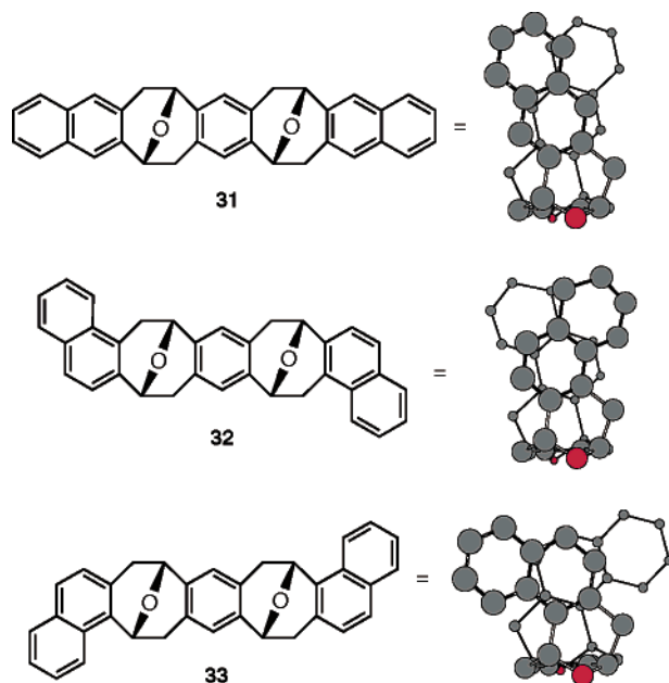
FIGURE 15. Possible chiral molecular tweezers with naphthalene pincers.
