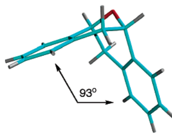
FIGURE 4. Crystal structure of Kagan's ether.
